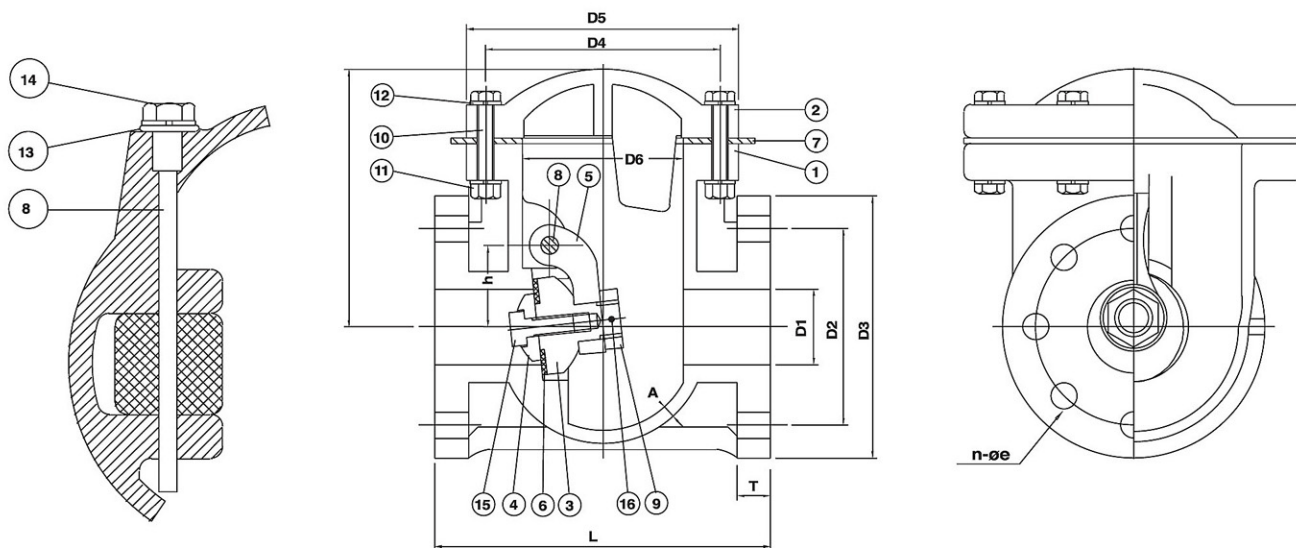
DN25~DN200
